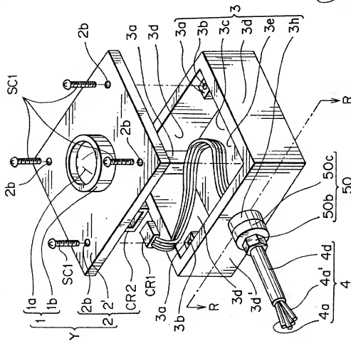
PRIOR ART FIG. 11
